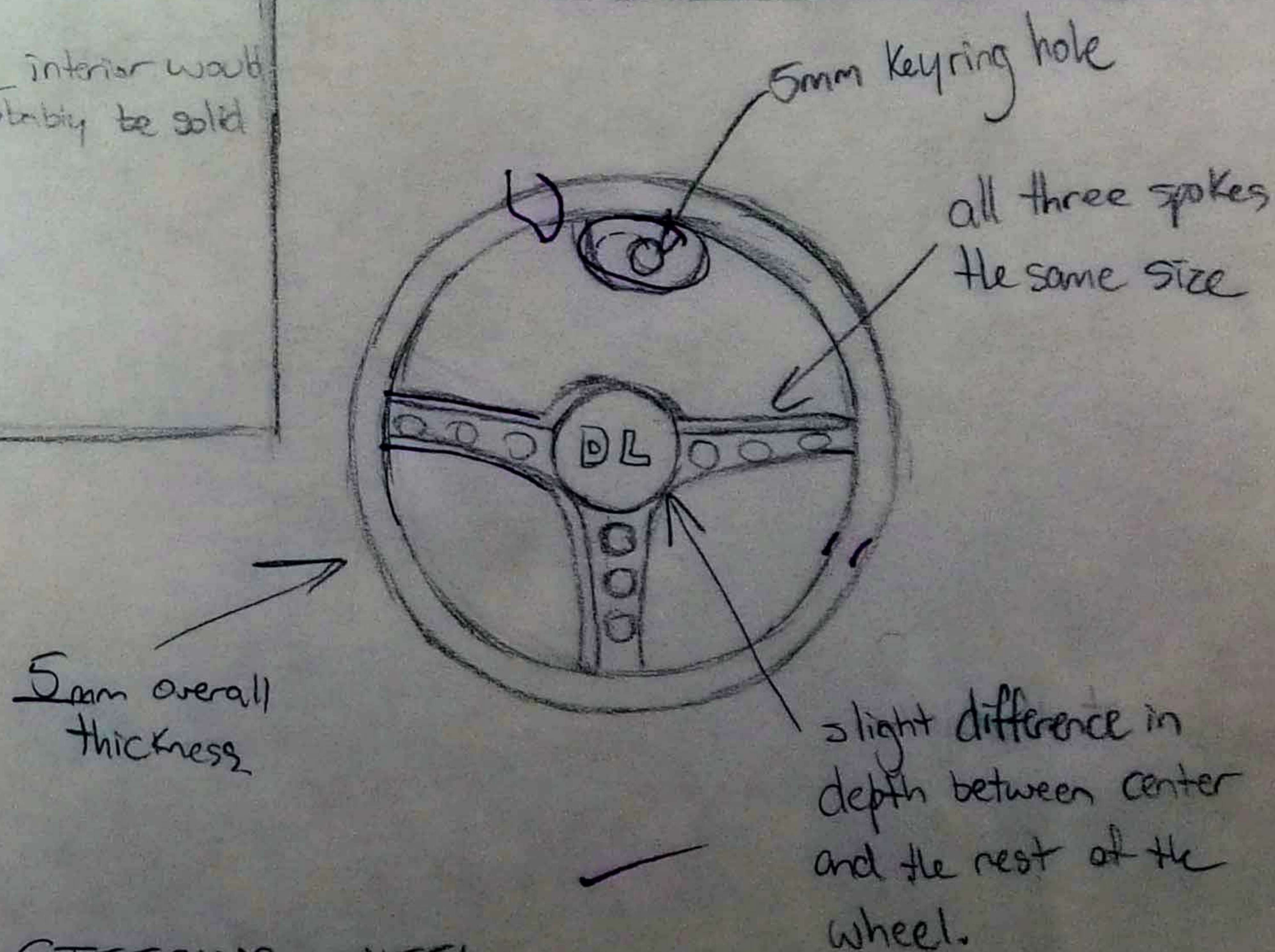
STEERING WHEEL
